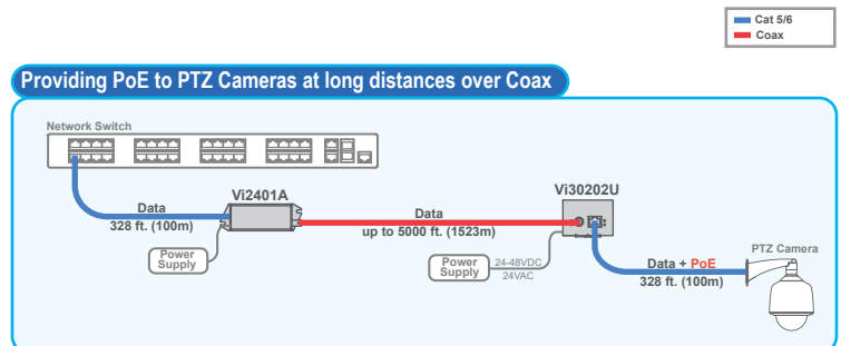
Vi30202U along with Vi2401A can be used to provide data and PoE transmission over long distance coax cables.
